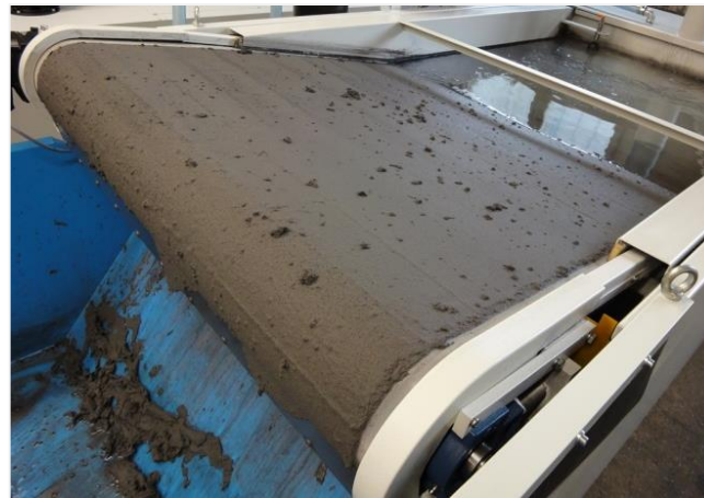
Picture 4: GKD's self-cleaning MAXFLOW stainless steel belt.
