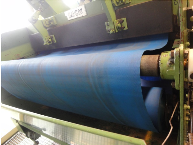
Picture 1: The highly permeable VACUBELT® 3354 polyester filter belt offers greater cooling lubricant filtration security.
